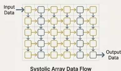
Systolic Array Data Flow
